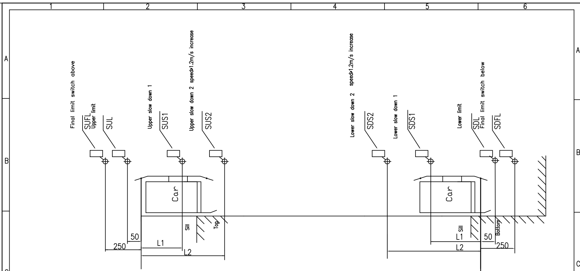
The installed distance of speed corresponding switch
